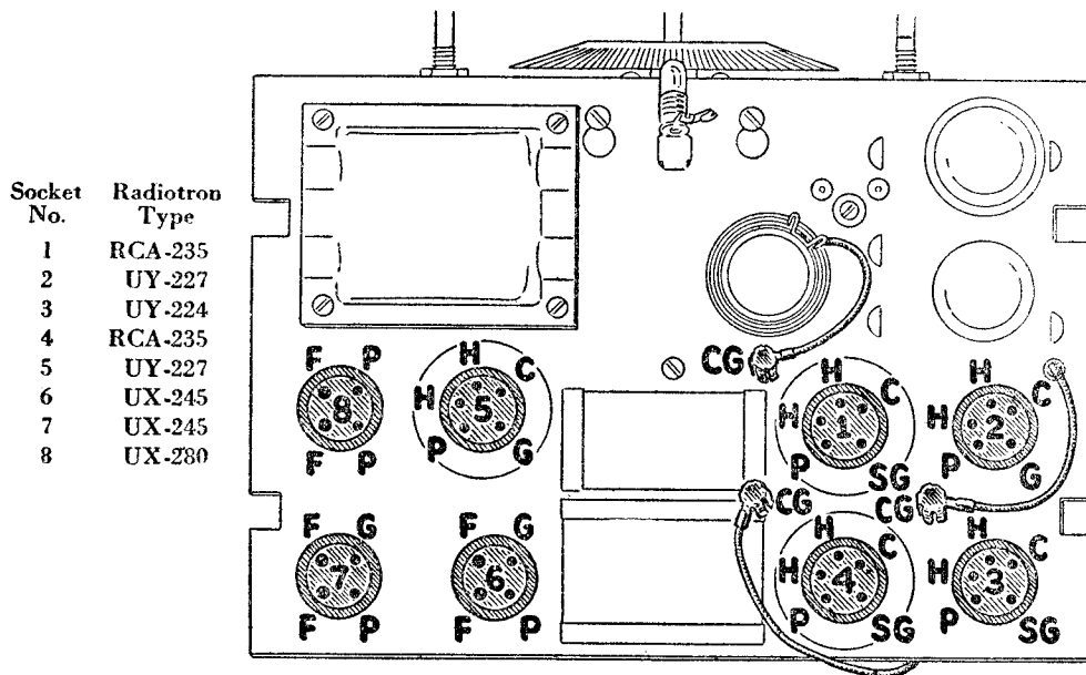
Figure 3—Socket Location and Contact Position of Receiver Assembly
